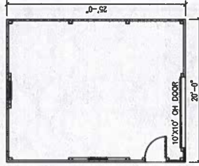
PLAN 1/8" = 1'-0" N
